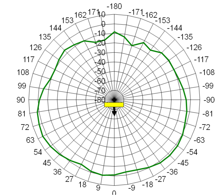
WLAN 2400 MHz Peak Gain: +4 dBi
