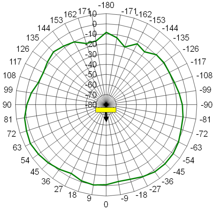
WLAN 2400 MHz Peak Gain: +4 dBi
