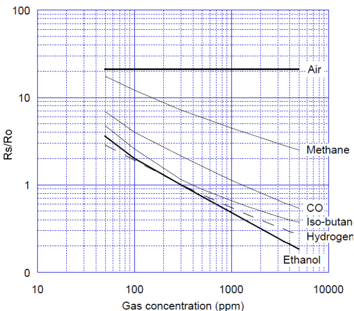
Sensitivity Characteristics:
