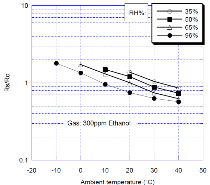
Temperature/Humidity Dependency:
