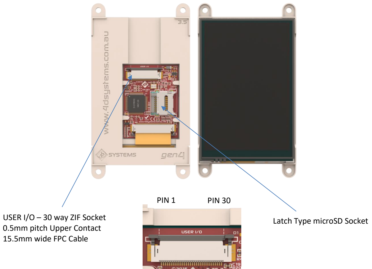
USER I/O – 30 Way FPC
