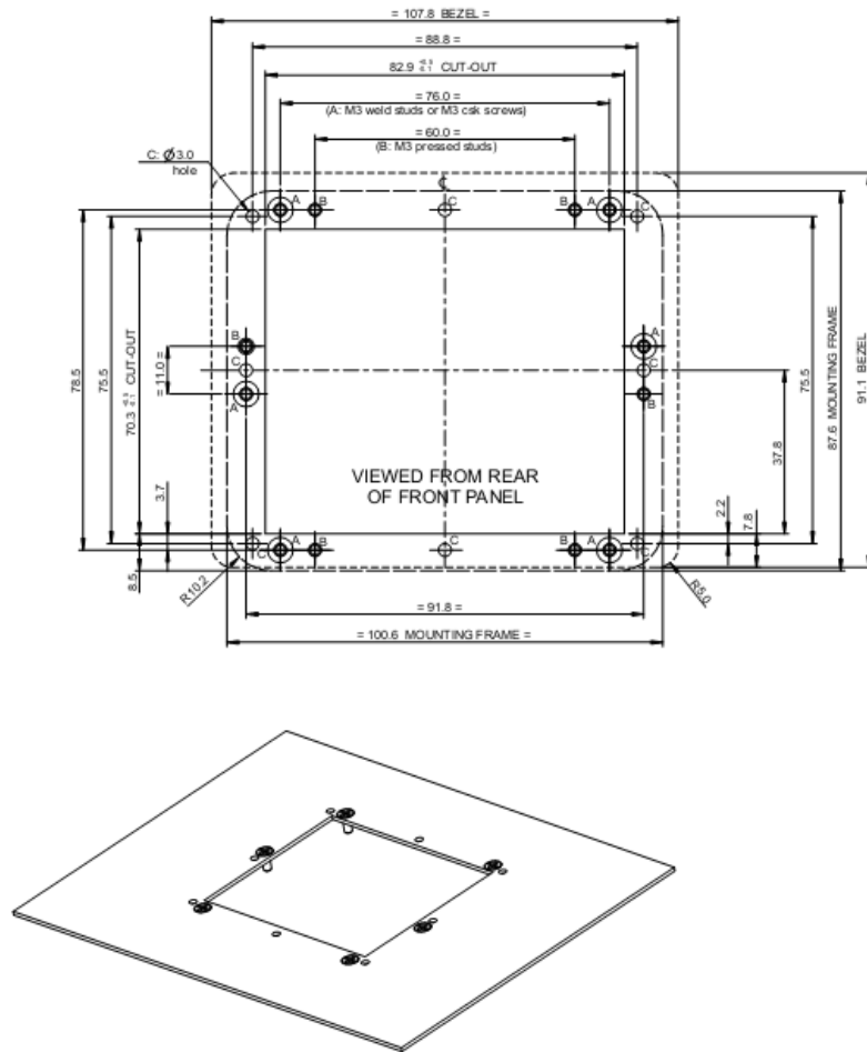
Figure 5.3 VM800P 3.5" panel mount dimensions
